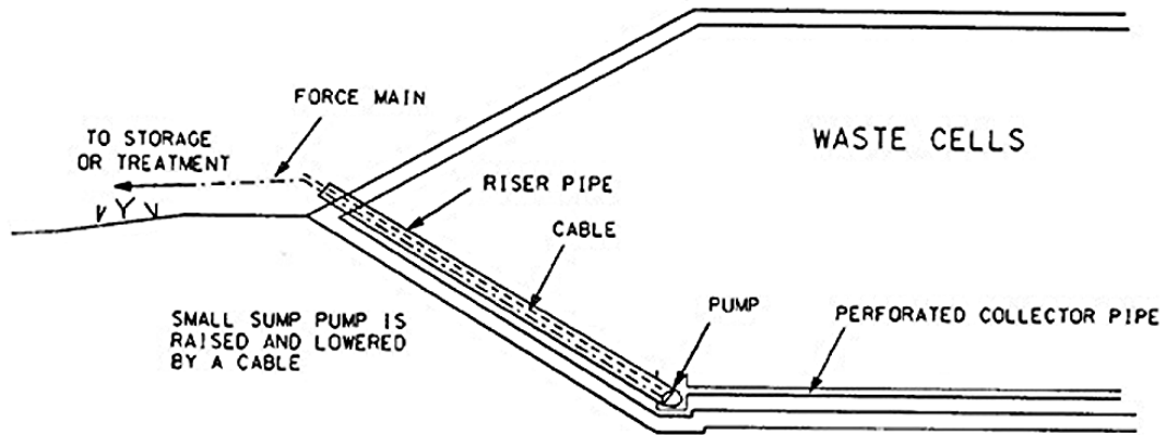
Figure 11 Collection Systems with Riser Pipes
