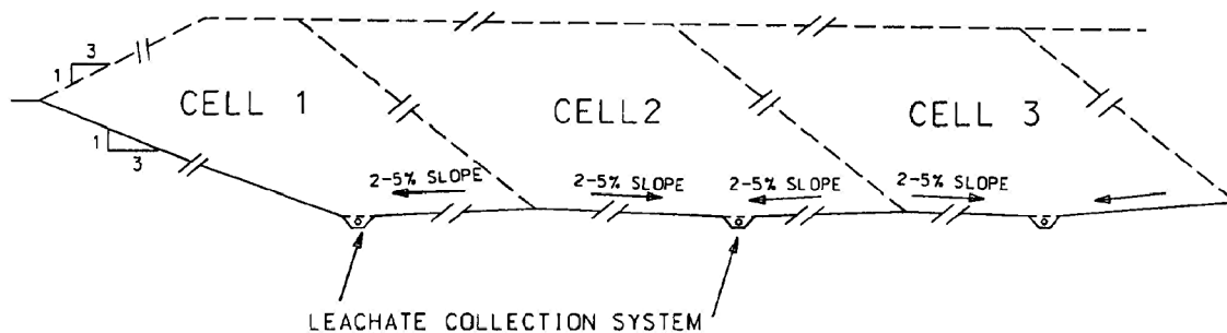
Figure 5 Alternate Trench Bottom Design
