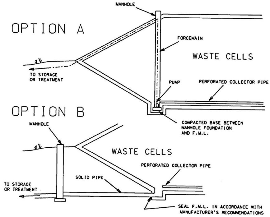
Figure 10 Collection Systems with Manholes
