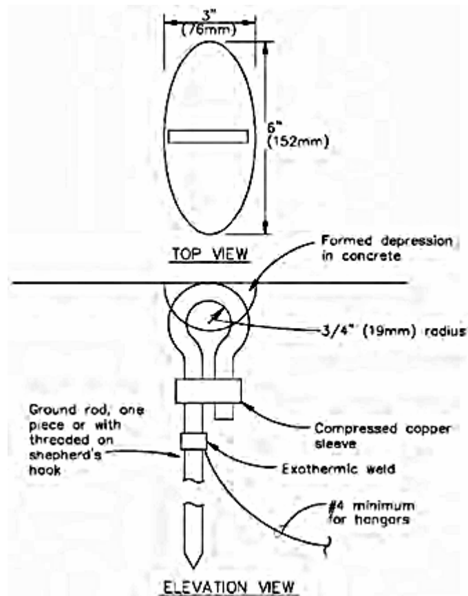
Figure 2.2 Static Grounding Point.
