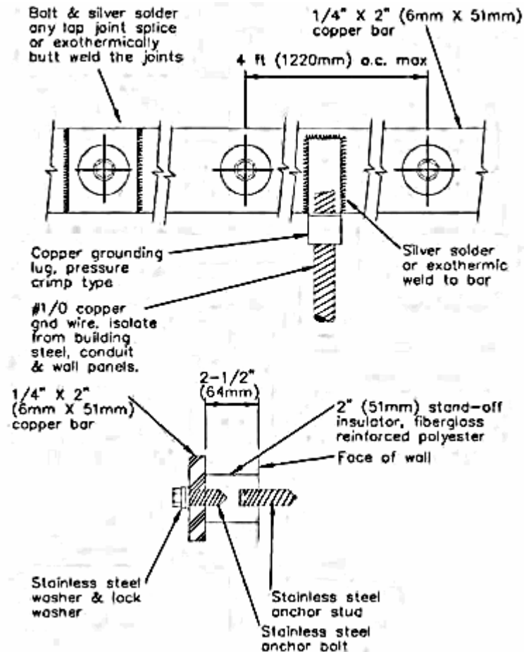
Figure 2.1 Static Bus Bar
