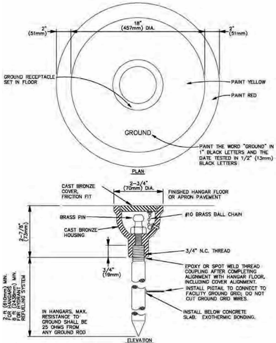
Figure 2.3 Grounding Receptacle.
