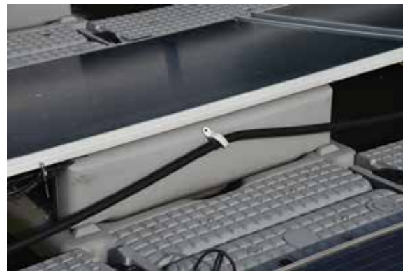
FIGURE 7.7 Clamps used to guide cables along the upper surface of floats
