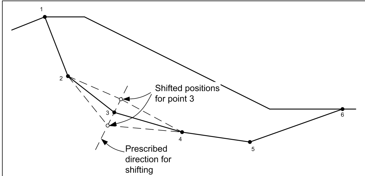
Figure C-8. Search scheme for noncircular slip surfaces (after Celistono and Duncan 1981)
