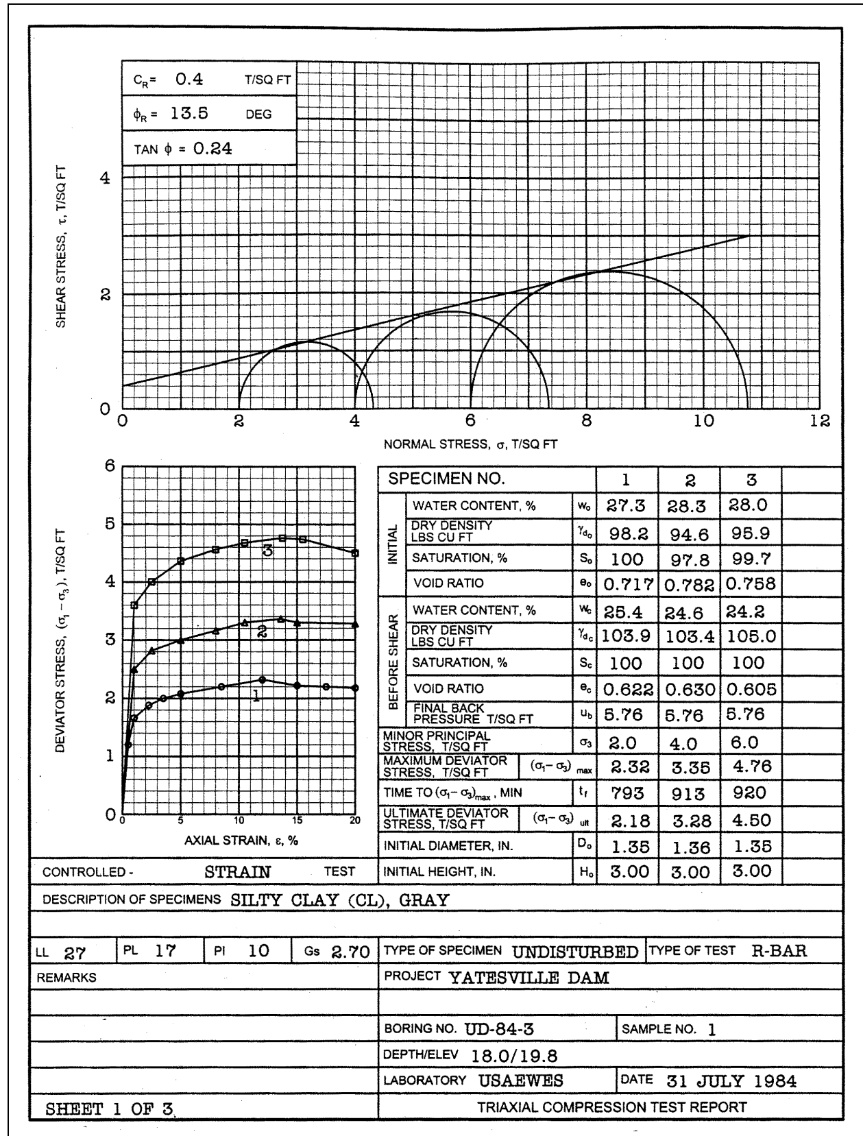
Figure 4-6. Triaxial compression test report for R-bar (consolidated-undrained) tests – total stress envelope
