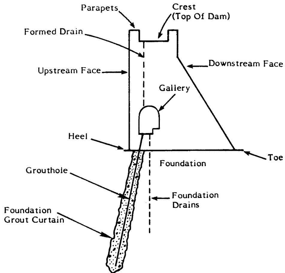
FIGURE I-7. CROSS-SECTION OF GALLERY SHOWING LOCATION OF TYPICAL DRAINS AND GROUT CURTAIN (Elevation View)
