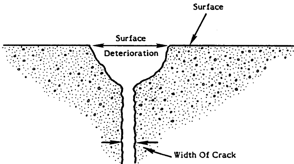
FIGURE II-1. DETERMINING CRACK WIDTH (Sectional View)
