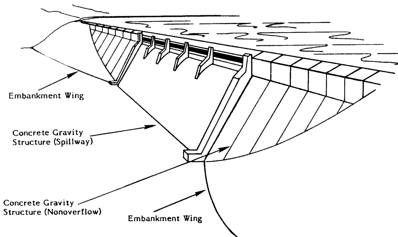
FIGURE I-4. COMPOSITE DAM
