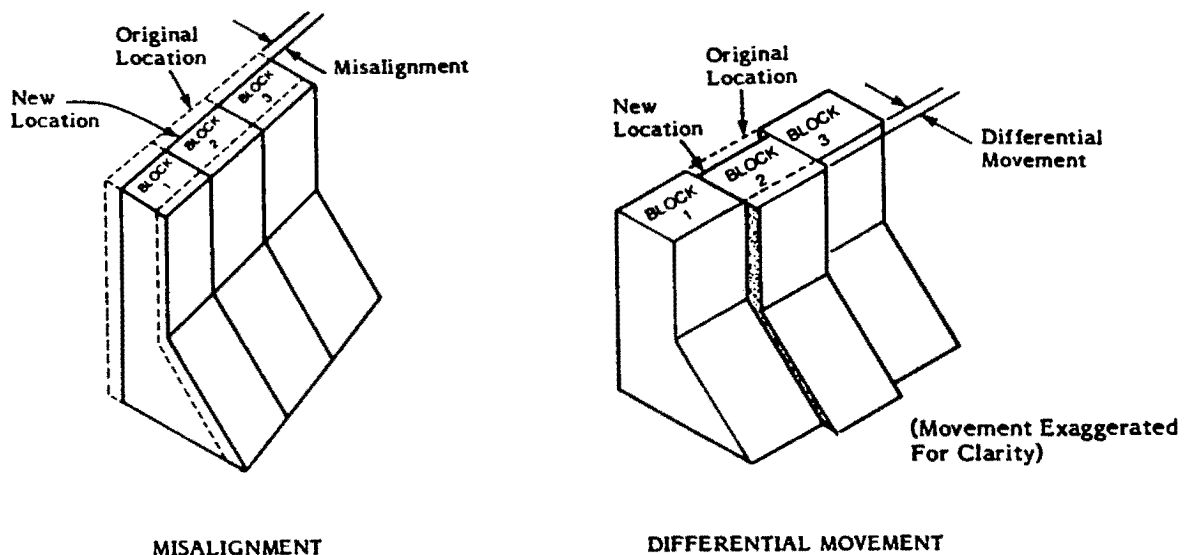
FIGURE II-14. MISALIGNMENT AND DIFFERENTIAL MOVEMENT
