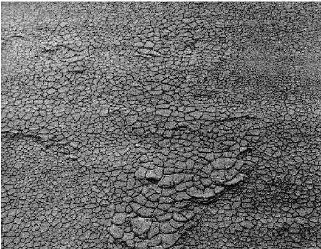
Figure 16. Severe alligatoring on thick coating of asphalt.
