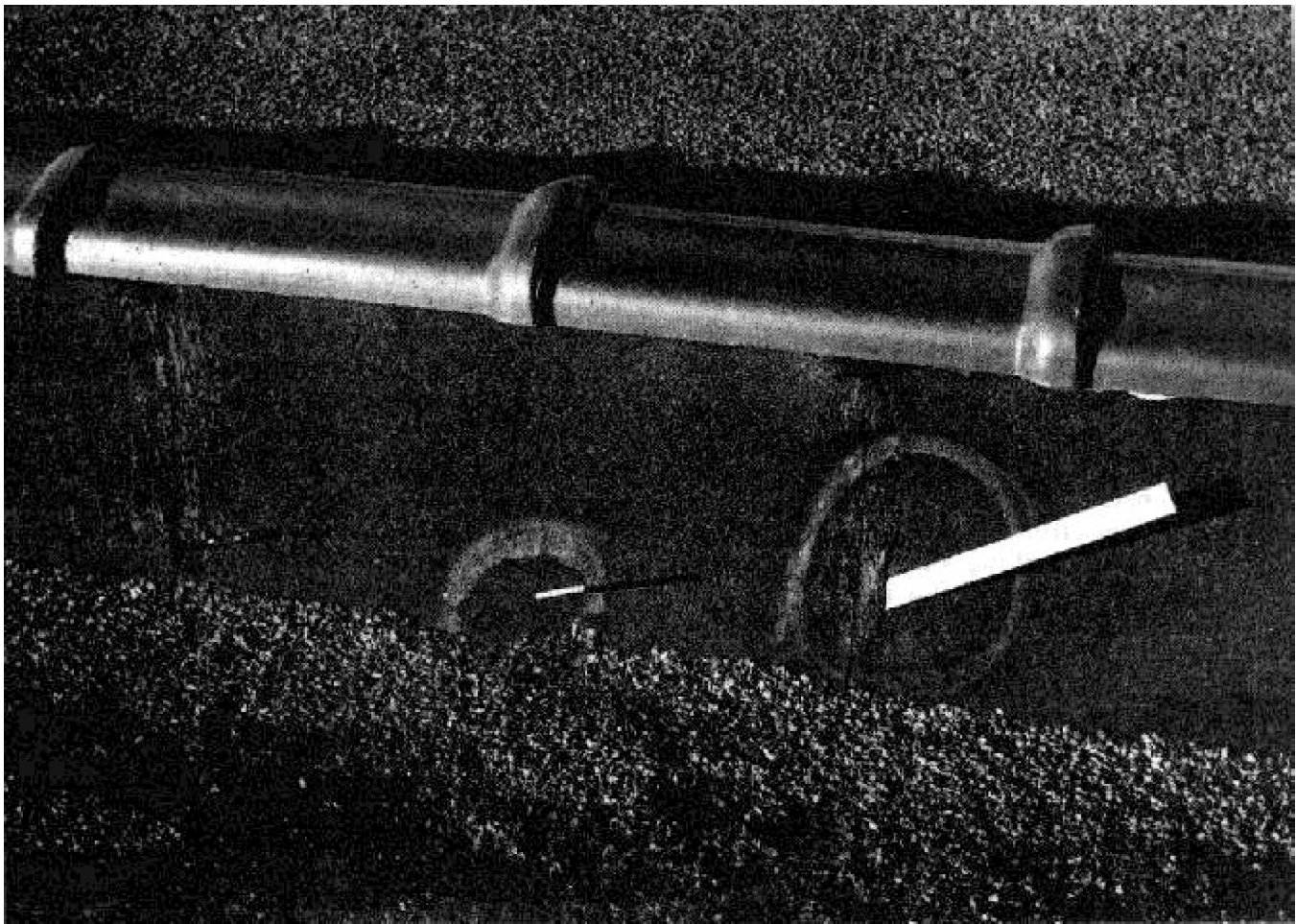
Figure 49. Open laps and split in base flashing..
