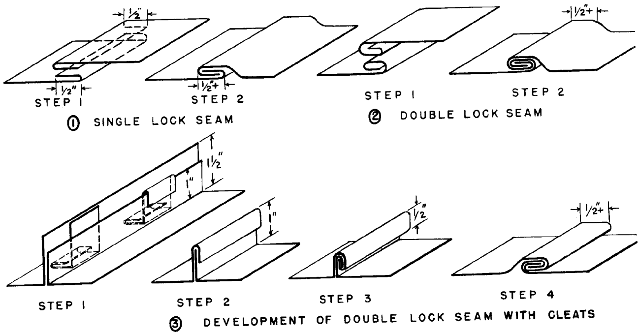
Figure 43. Development of lock seams.
