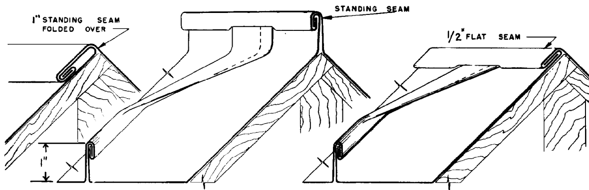
RIDGE DETAILS
