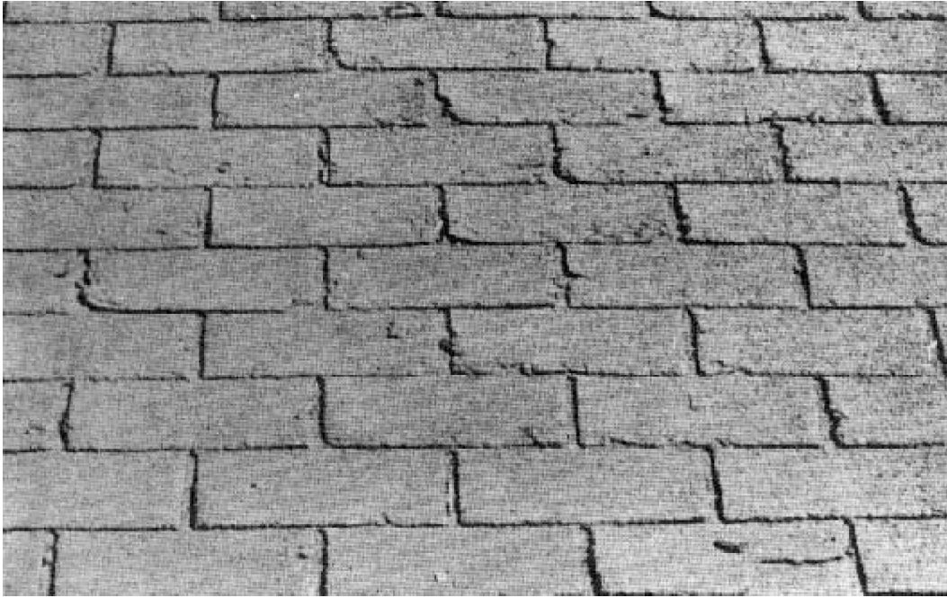
Figure 27. Recoated asphalt shingles — note damage resulting from brittleness.
