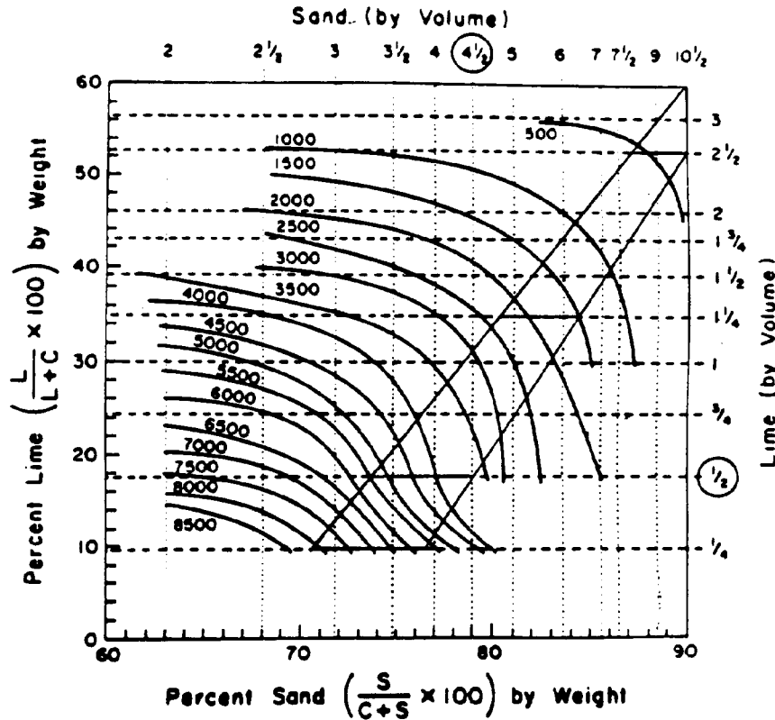
Figure 3-3. Strength of mortar (psi) versus constituent proportions.
